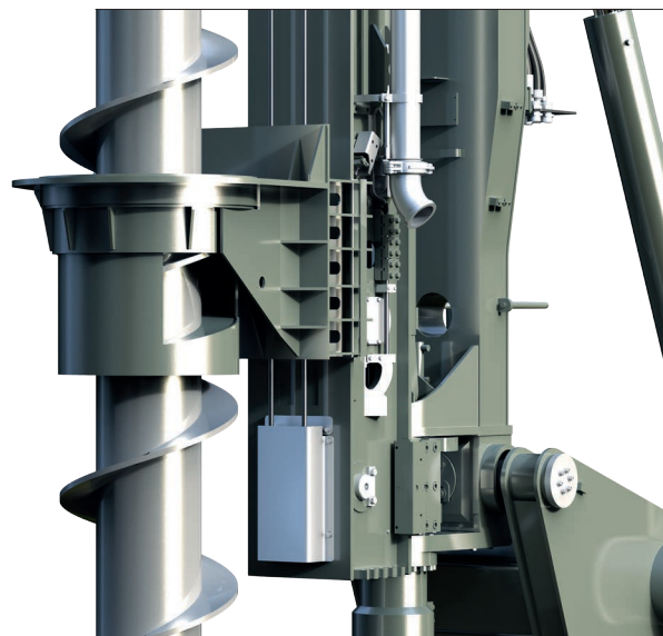
Auger with hydraulic auger cleaner
